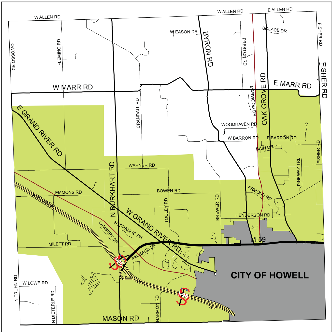
MAP NO. 29 PLAN FOR SANITARY SEWER
