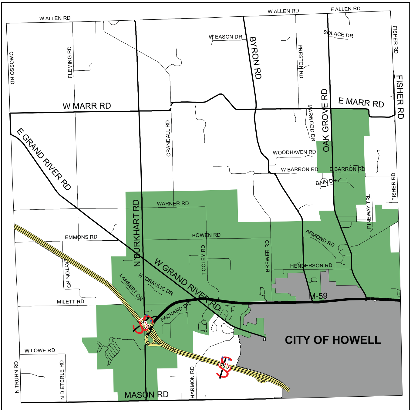
MAP NO. 19 SANITARY SEWER SYSTEM AND SERVICE AREA
